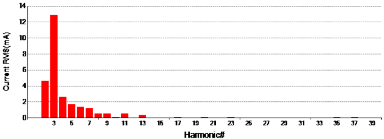
Harmonics Histogram
